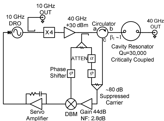
Figure 2. Block diagram of the cavity stabilized oscillator (CSO) at 40 GHz. The 10 GHz DRO is phase-locked to the phase-transfer function of the air-cavity resonance. DBM is double-balanced mixer, ATTEN is attenuator and \beta_1 is input coupling.
