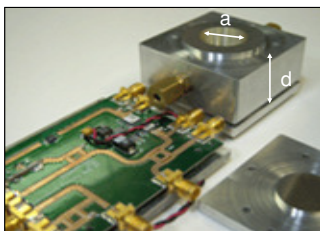
Figure 1. Air-dielectric cylindrical Al cavity resonator at 40 GHz. The diameter (a) and the length (d) of the cavity are approximately 2 cm.
