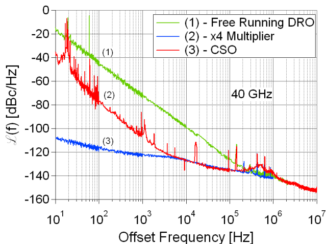
Figure 4. PM noise of a cavity stabilized oscillator (CSO), the results are normalized to 40 GHz. One sees the significant noise reduction of the free-running DRO noise out to beyond 100 kHz offset frequency.
