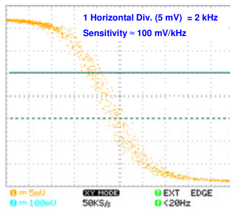
Figure 3. Typical error signal from the double balanced mixer (DBM) in the cavity discriminator of Fig. 2 measured by an oscilloscope. One division along the x and y-axis is equal to 5 mV and 100 mV, respectively. 5 mV along x-axis corresponds to a frequency error of 2 kHz between the (10 GHz \times 4) DRO and the cavity resonance frequency.
