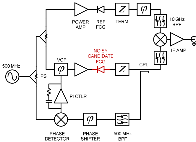
Figure 2 - Block diagram of experimental measurement setup. Items are abbreviated as: Power Splitter (PS), Reference (REF), Voltage Controlled Phase Shifter (VCP), Directional Coupler (CPL), Proportional-Integral Controller (PI CTRL) and FCG attenuator/isolator termination (TERM).
